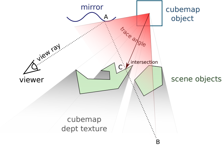
Figure 3.1: Principle of the cubemap tracing algorithm, using one CMO. The reflected view ray is iteratively traced along an angle defined by the mirror-incidence point (A) and a distant point of the ray (B). The goal is to find the intersection with scene objects (C), which is possible because of the objects being captured in the cubemap depth texture.
